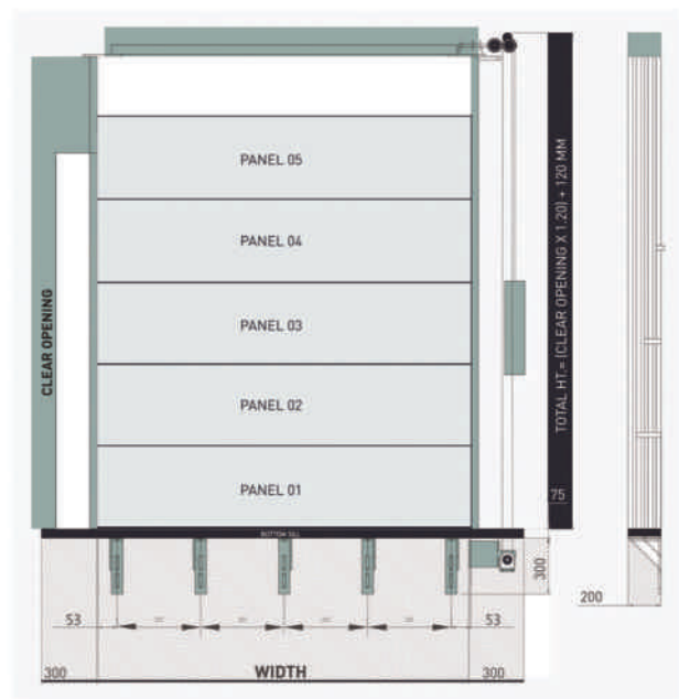
5 panel vertical door
